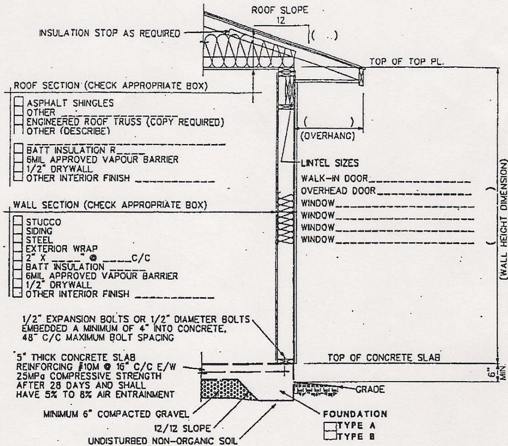
TYPICAL WALL/ROOF SECTION NOT TO SCALE
